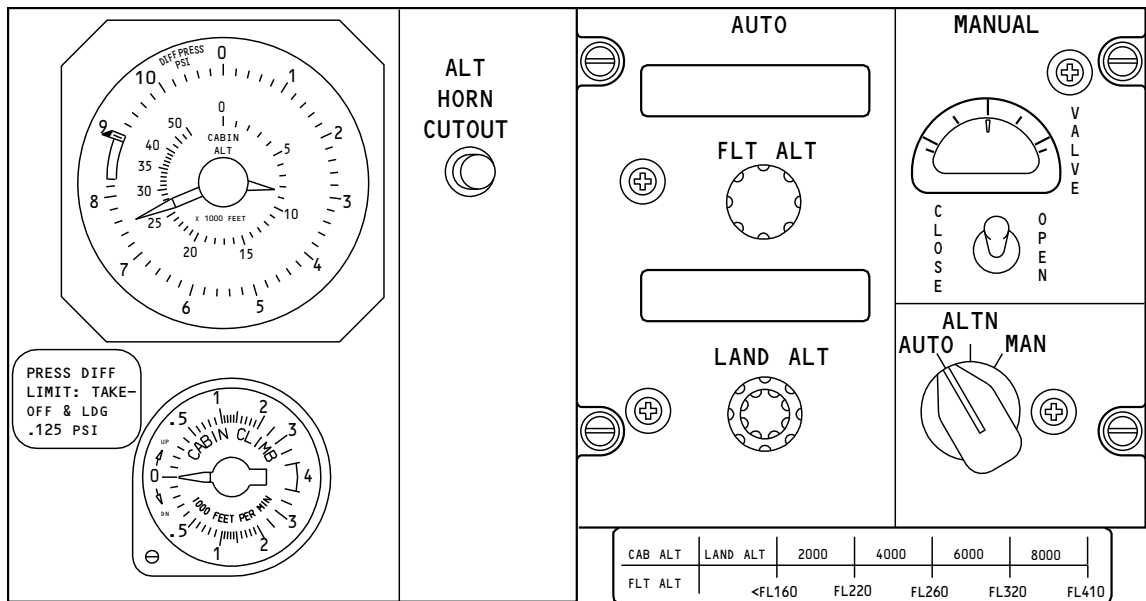
CABIN ALTITUDE PANEL
