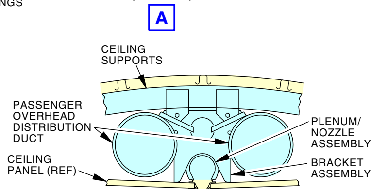
OVERHEAD DISTRIBUTION DUCT INSTALLATION
