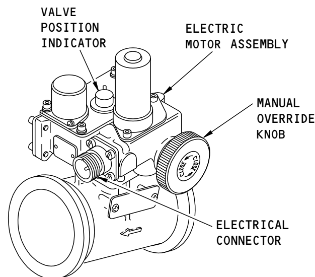
ZONE TRIM AIR MODULATING VALVE (EXAMPLE)
