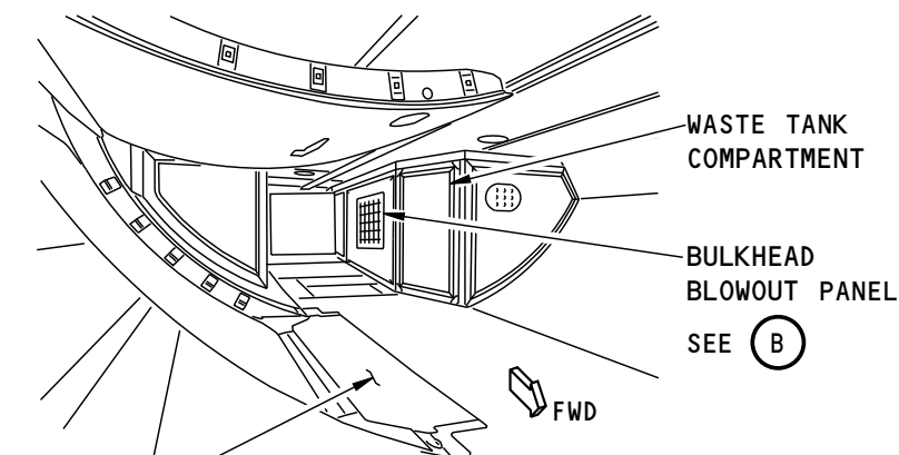
AFT CARGO COMPARTMENT
