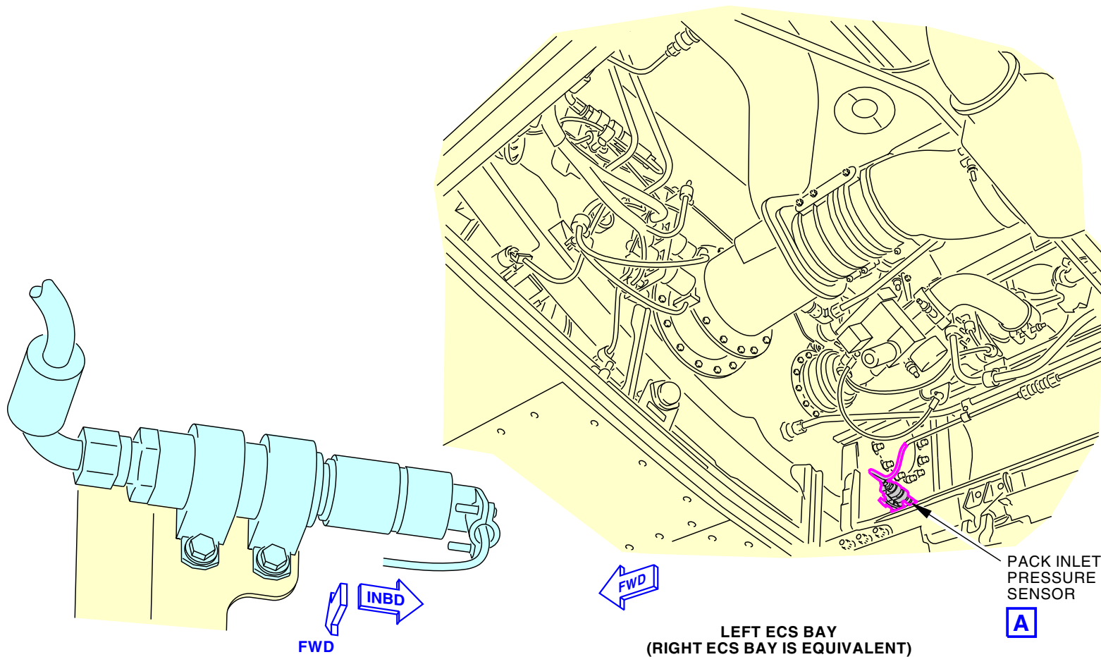
PACK INLET PRESSURE SENSOR
