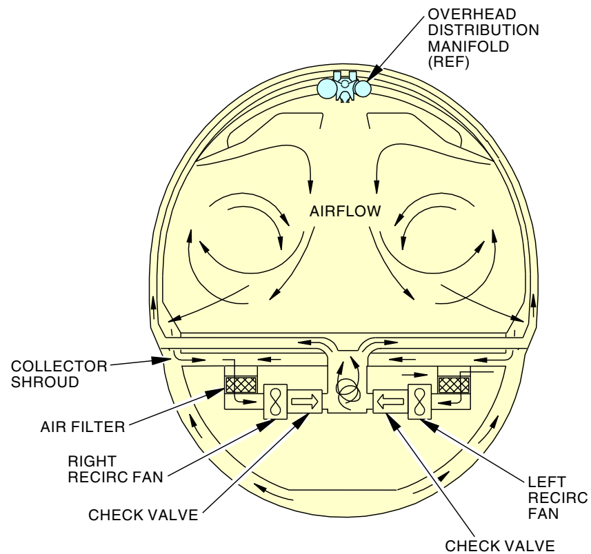
RECIRCULATION SCHEMATIC
