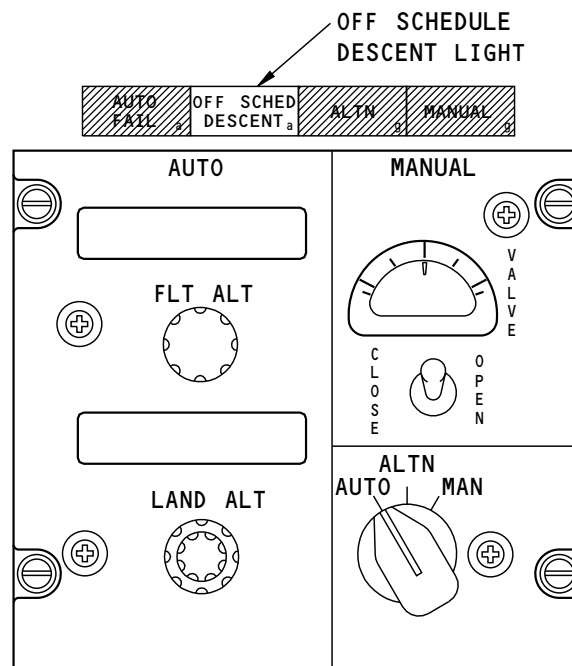
CABIN PRESSURE CONTROL MODULE (P5)
