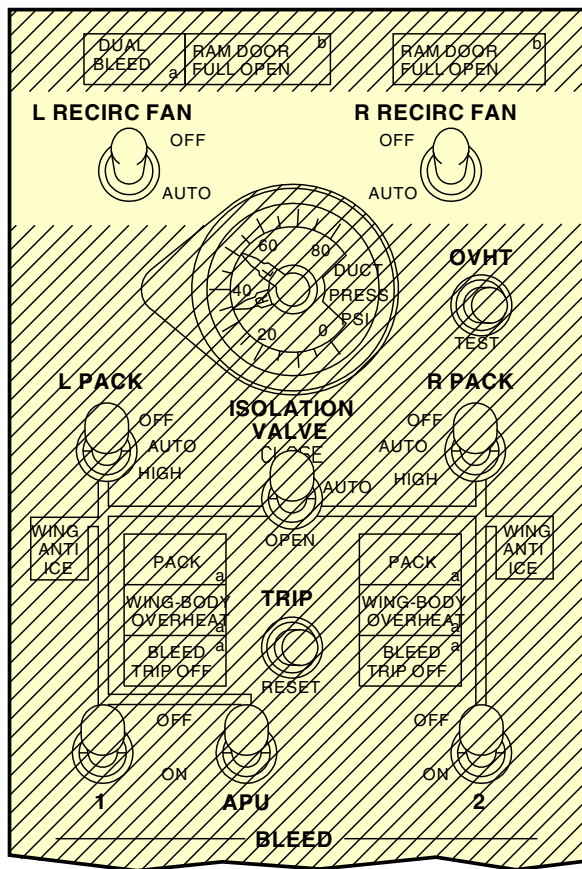
AIR CONDITIONING/BLEED AIR CONTROLS PANEL (P5)
