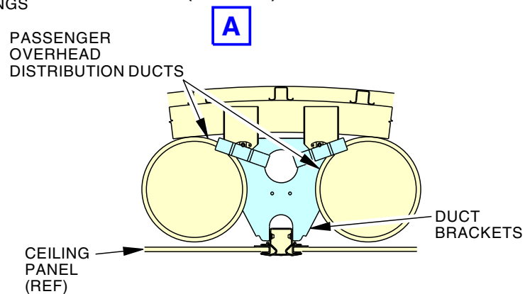
OVERHEAD DISTRIBUTION DUCT INSTALLATION
