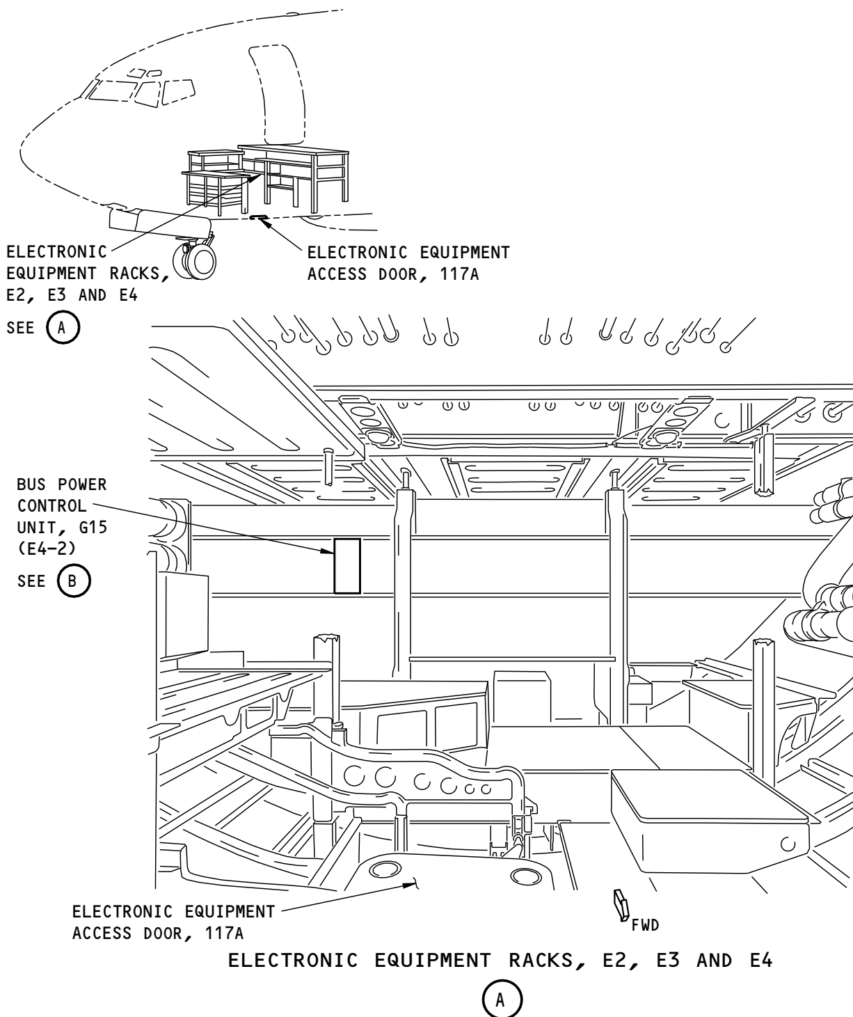
Bus Power Control Unit (BPCU), G15 Figure 201/24-41-00-990-802 (Sheet 1 of 2)
