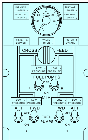
FUEL CONTROL PANEL
