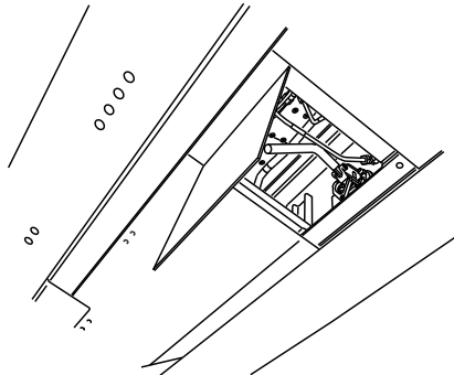
DEFUEL VALVE
