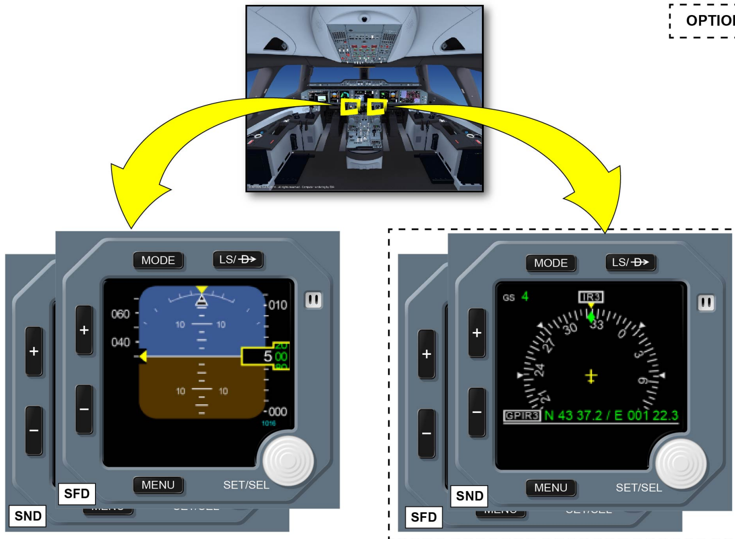
INTEGRATED STANDBY INSTRUMENT SYSTEM (ISIS) (2/3)
