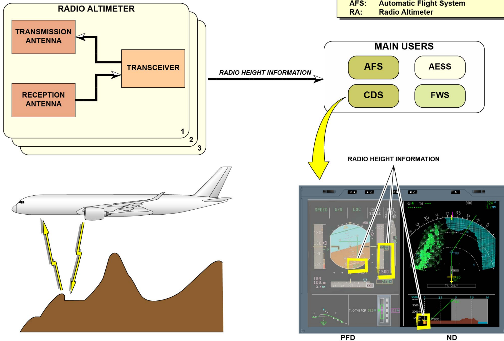
RADIO ALTIMETER: GENERAL
