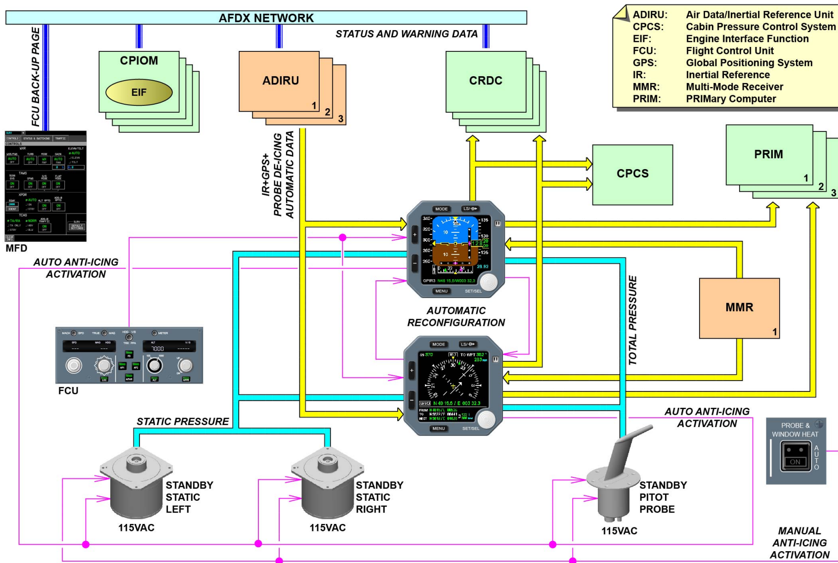
STANDBY NAVIGATION SYSTEM INTERFACES - INTERFACE BETWEEN THE TWO ISIS (DUAL CONFIGURATION) ... PROPULSION CONTROL SYSTEM (PCS)
