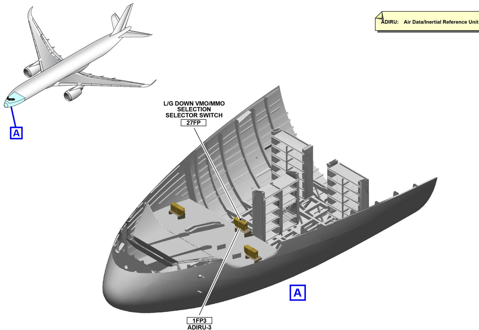
ADIRS START PROCEDURE (ALIGN ON GPS POSITION) (2) ... NAIADS OPERATION (3)
