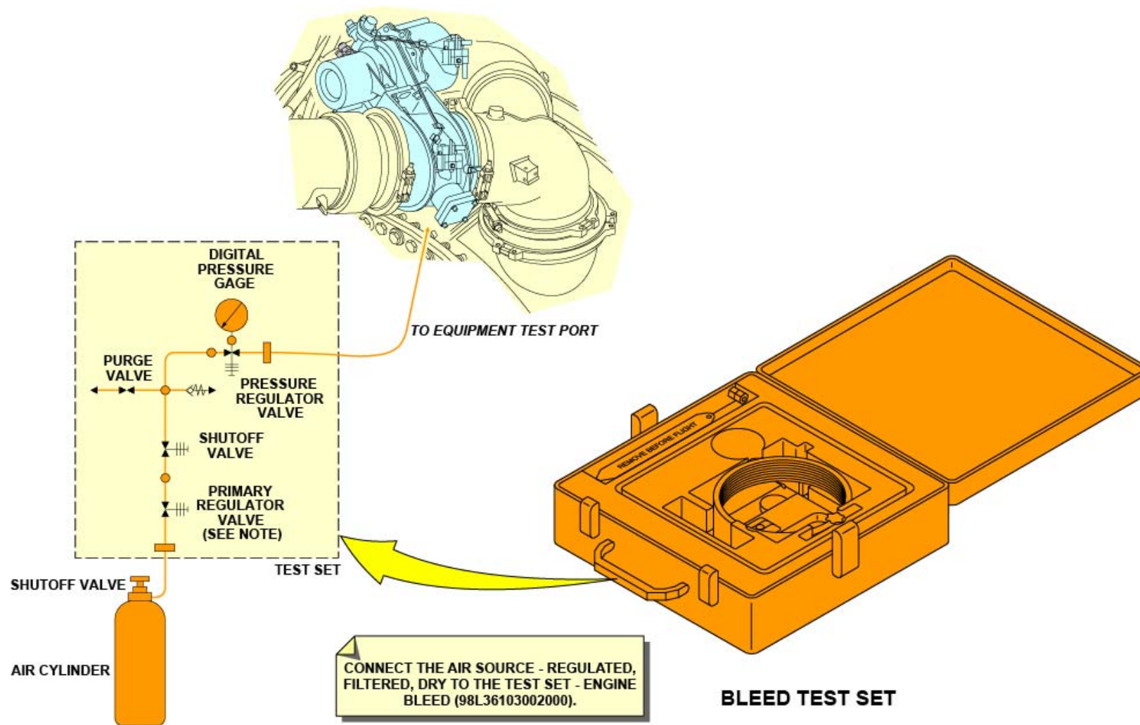
TOOLS - BLEED TEST SET
