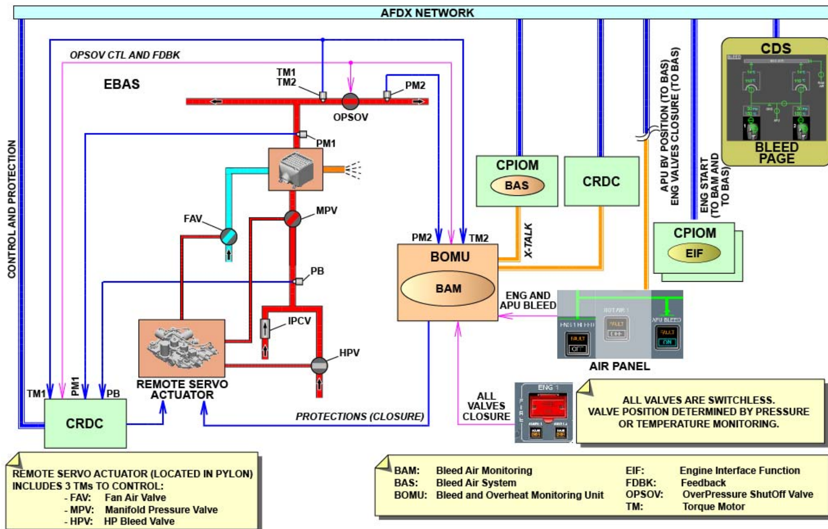
EBAS SYSTEM FUNCTION AND DESCRIPTION &amp; EBAS MONITORING AND INDICATING
