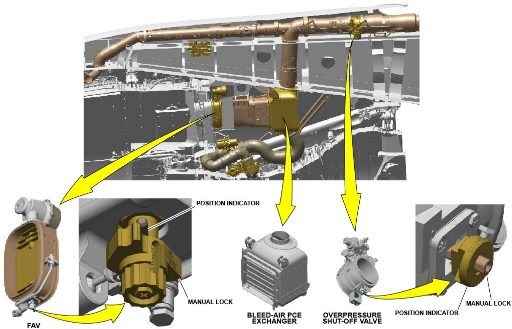
EBAS COMPONENTS DESCRIPTIONS - DEACTIVATION/REACTIVATION
