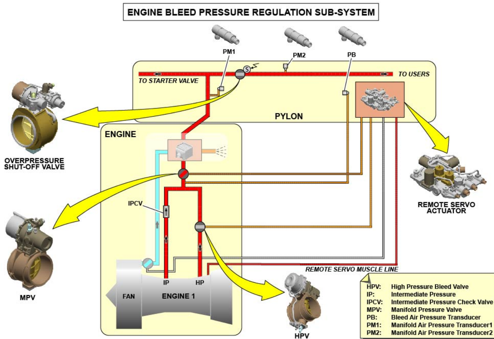
EBAS COMPONENTS DESCRIPTIONS - PRESSURE REGULATION SUB-SYSTEM COMPONENTS
