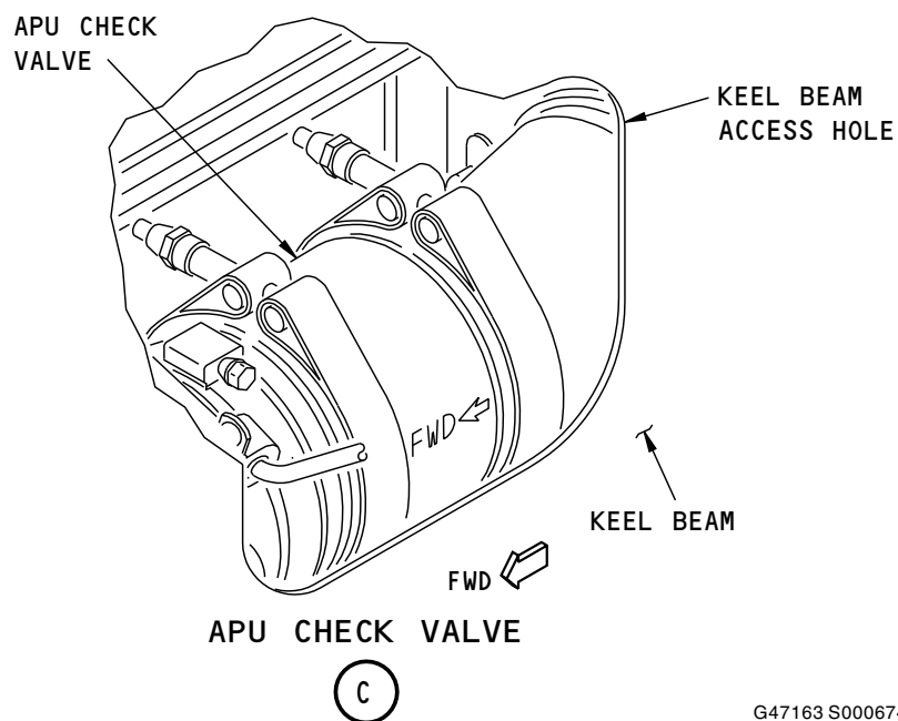
Pneumatic System in the Keel Beam Component Location Figure 303/36-10-00-990-803 (Sheet 2 of 2)
