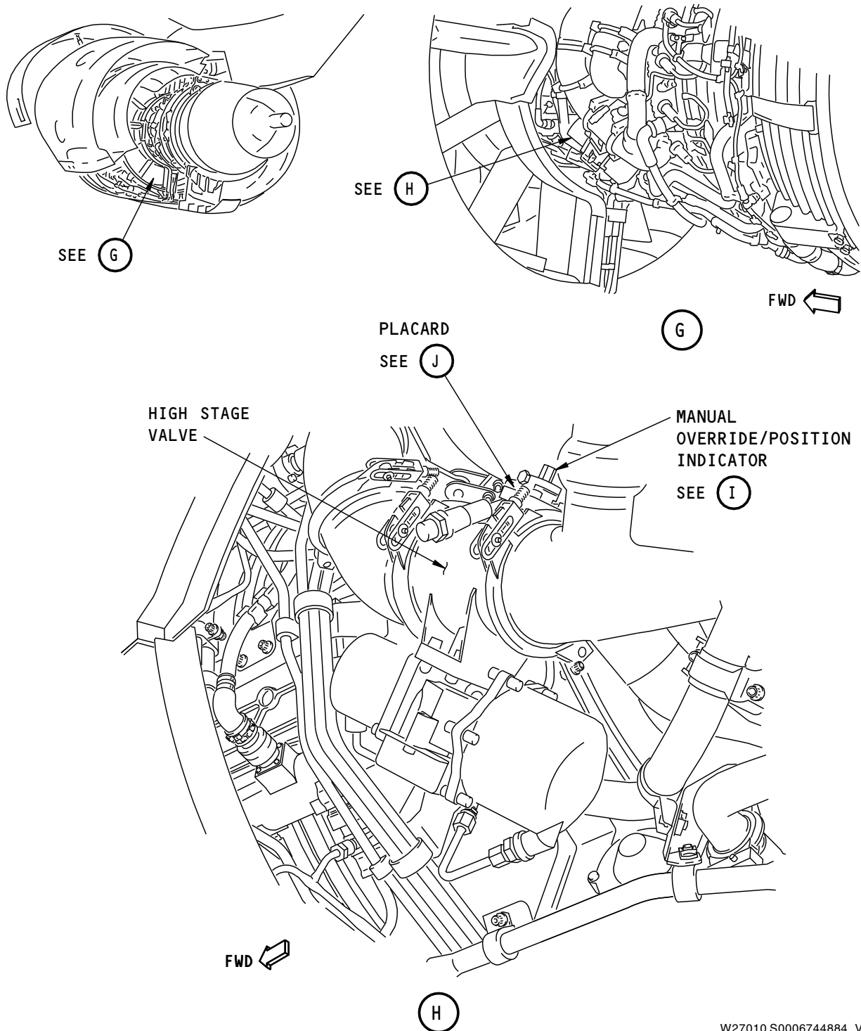
Pneumatic System Control Valve Position Indicators Figure 311/36-10-00-990-811 (Sheet 5 of 6)
