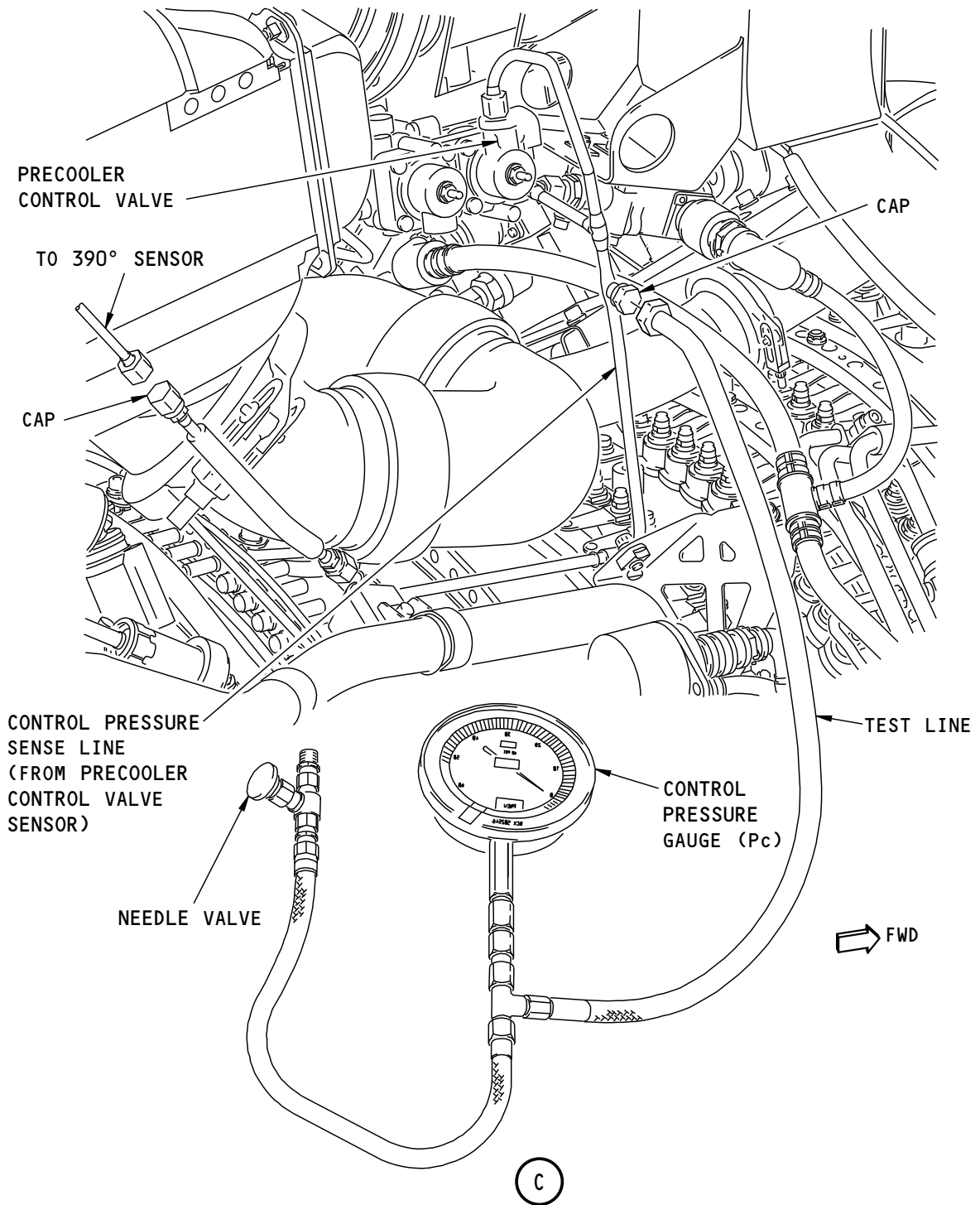
QUICK FIM TASK - Bleed Trip, the Engine is the Bleed Source Figure 312/36-10-00-990-813 (Sheet 3 of 3)
