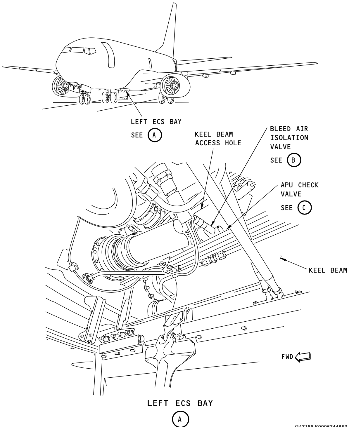
Pneumatic System in the Keel Beam Component Location Figure 303/36-10-00-990-803 (Sheet 1 of 2)
