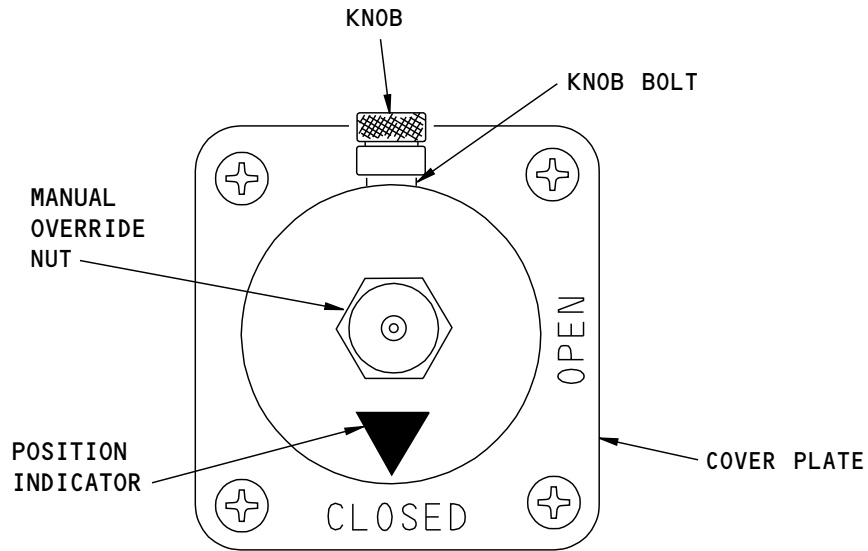
MANUAL OVERRIDE/POSITION INDICATOR
