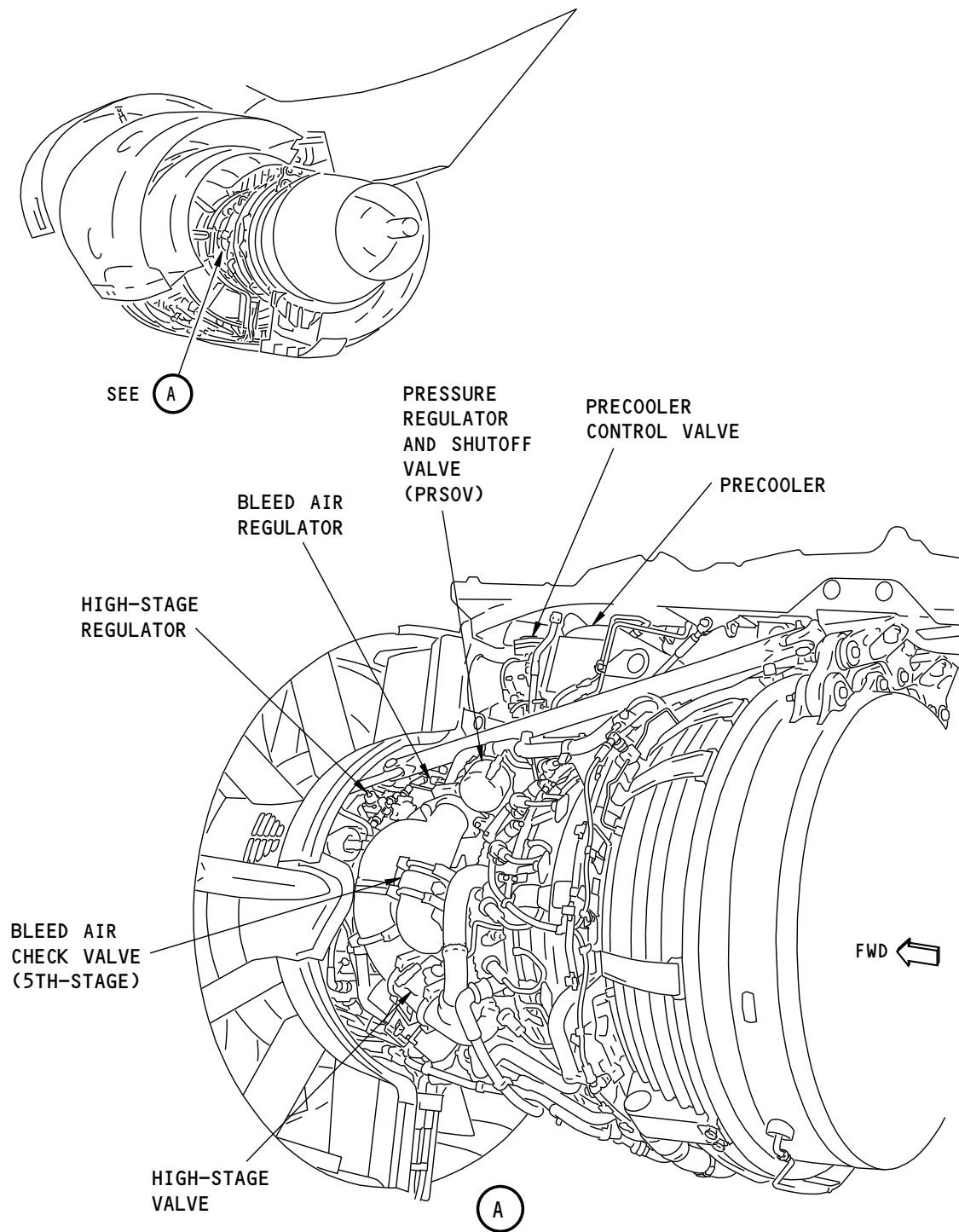
Pneumatic System on the Engine/Strut Component Location Figure 301/36-10-00-990-801 (Sheet 1 of 2)
