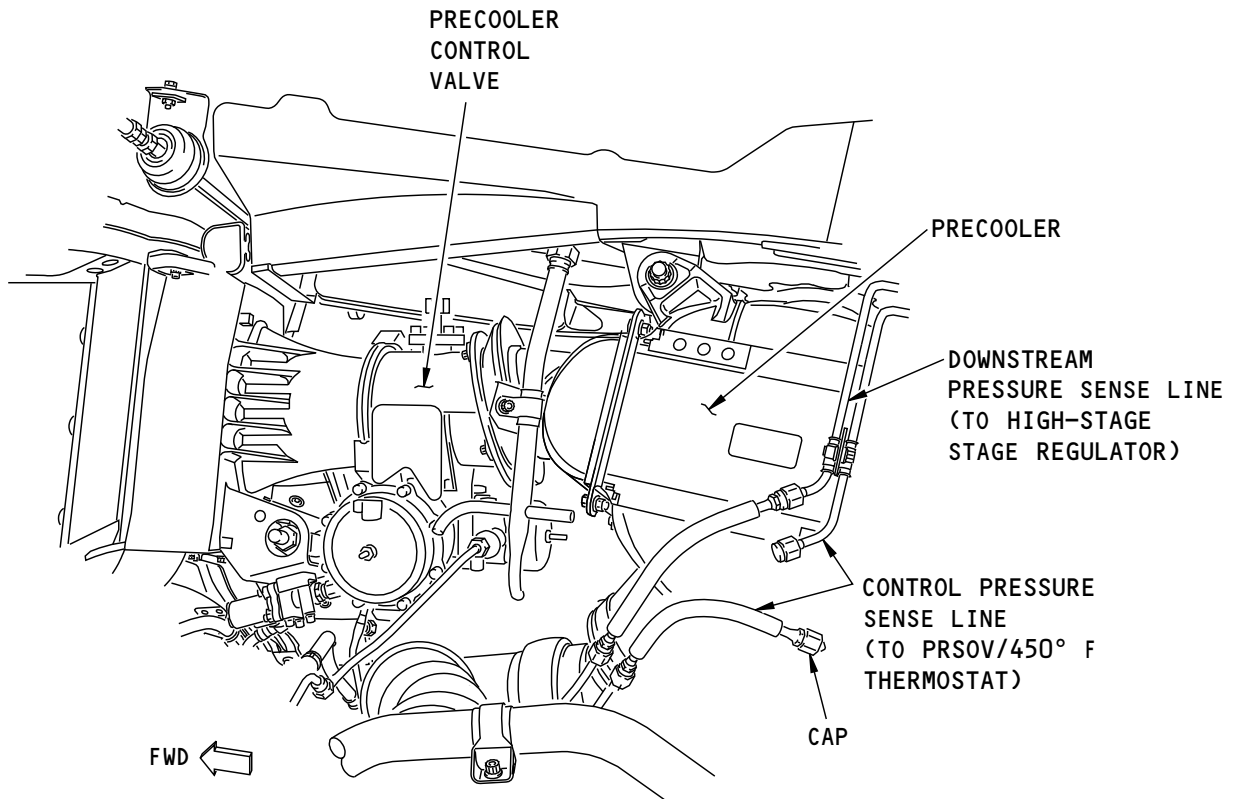
CONTROL PRESSURE SENSE LINE WITH CAP
