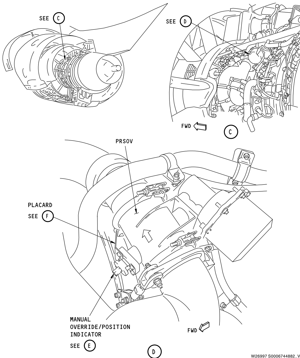
Pneumatic System Control Valve Position Indicators Figure 311/36-10-00-990-811 (Sheet 3 of 6)
