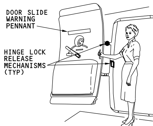
DOOR FULLY OPEN AND UPPER HINGE LOCKED
