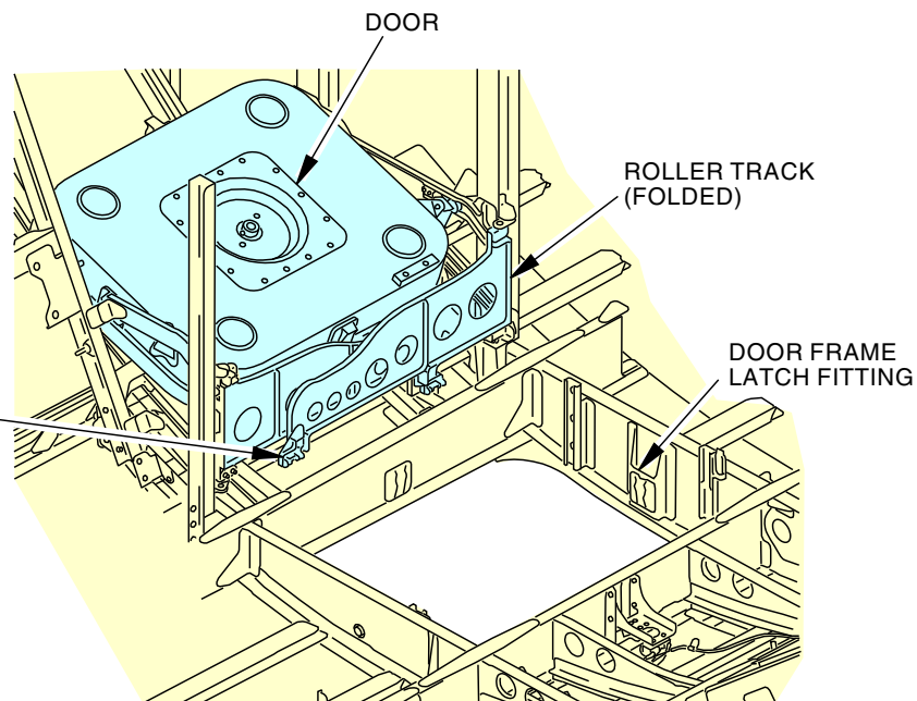
EE COMPARTMENT EXTERNAL ACCESS DOOR (INTERIOR VIEW - OPEN/ROLLER TRACKS FOLDED)
