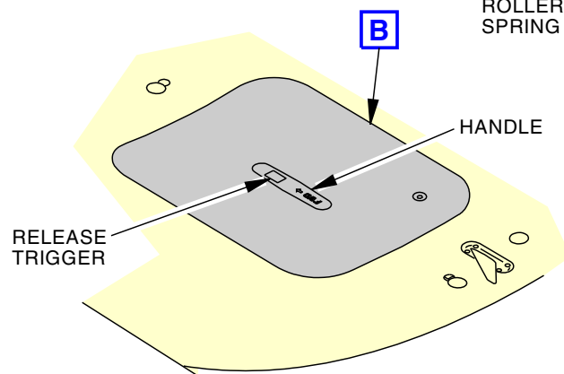
EE COMPARTMENT EXTERNAL ACCESS DOOR (EXTERIOR VIEW - CLOSED)
