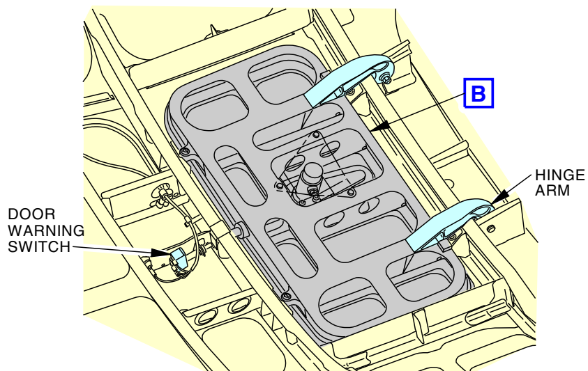
FORWARD EQUIPMENT COMPARTMENT ACCESS DOOR (INTERIOR VIEW - CLOSED)
