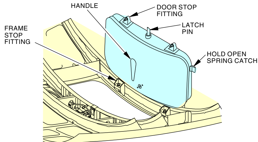
FORWARD EQUIPMENT COMPARTMENT ACCESS DOOR (INTERIOR VIEW - OPEN)
