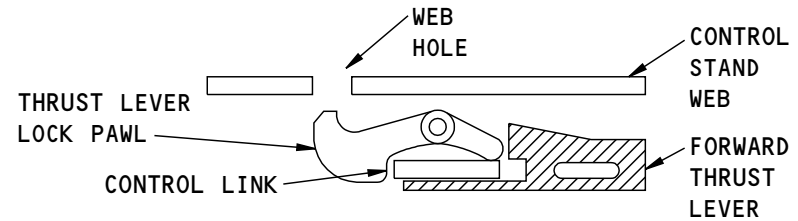
IDLE OPERATION
